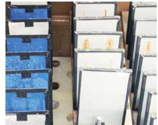
After 1,000 hours of alternating QUV/cyclic salt spray exposure testing Crystilium™ showed no signs of failure.
